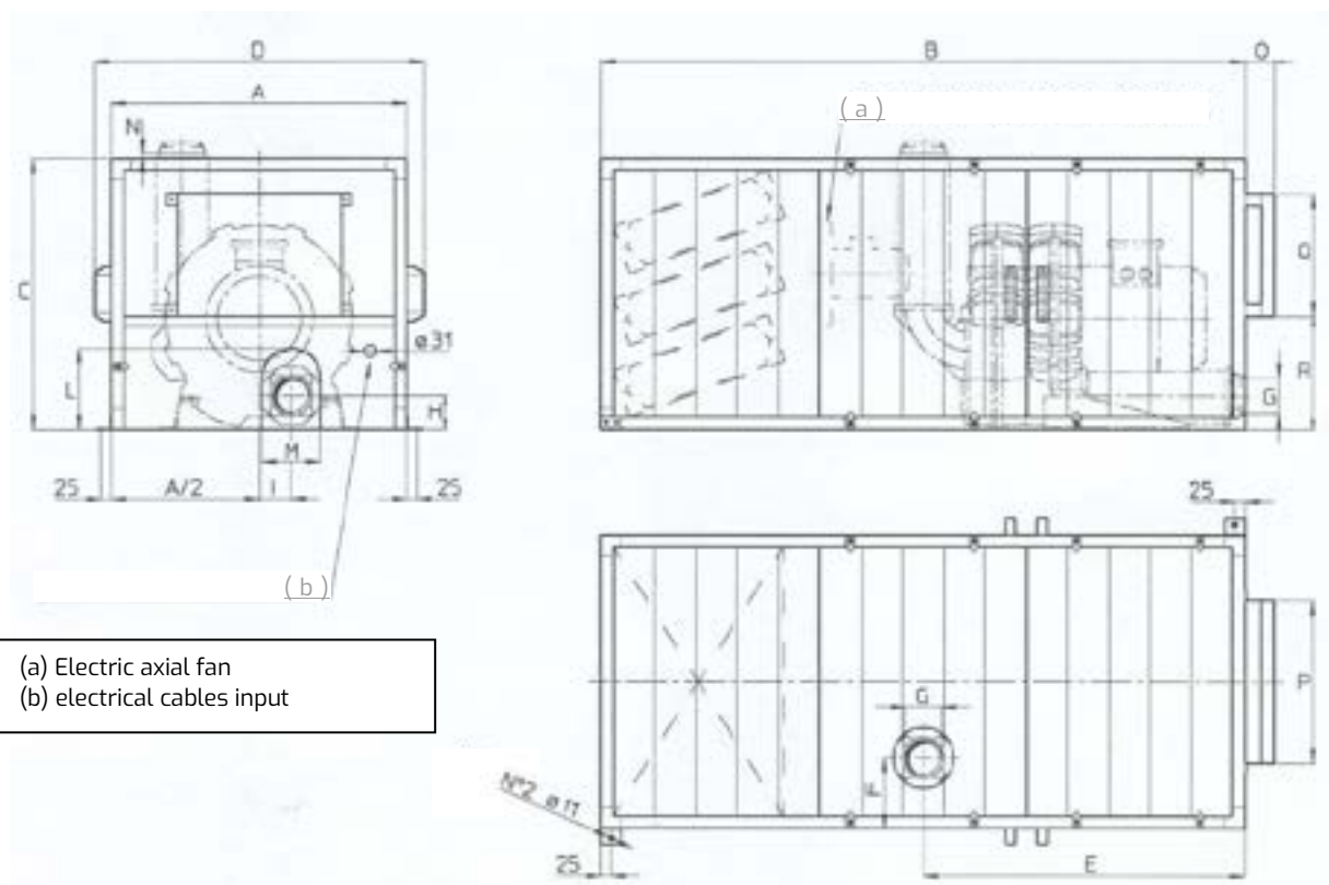
DIMENSIONS (IH8-IH11-IH12)
